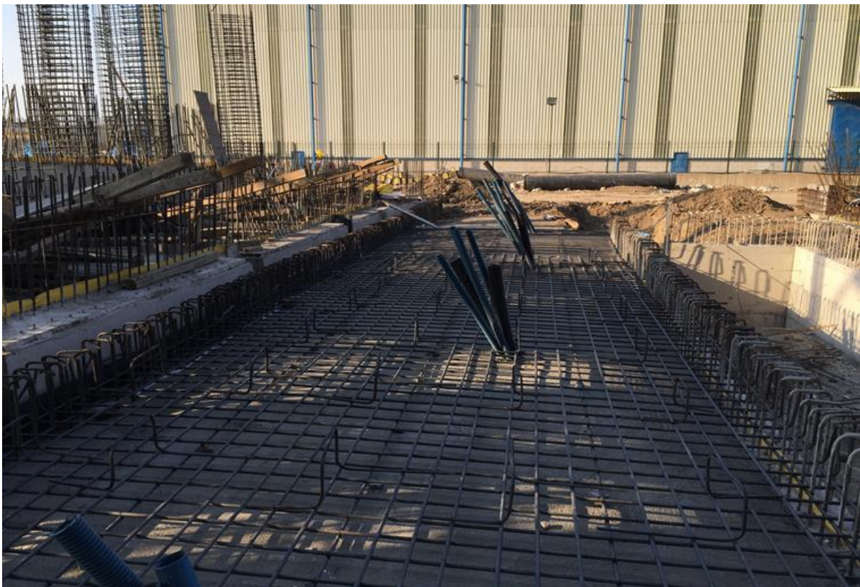
Pump and Instrument Power Supply Embedded Conduits
